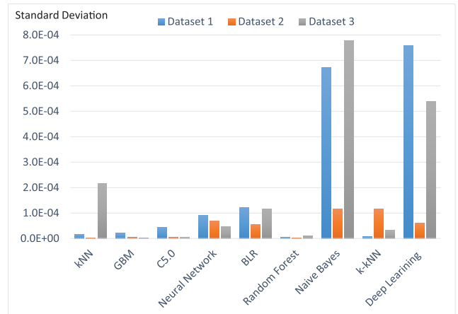
FIGURE 5. The Comparison of Accuracy of The Standard Deviation of All Algorithms with Evenly Distributed Dataset 1, 2 and 3.
