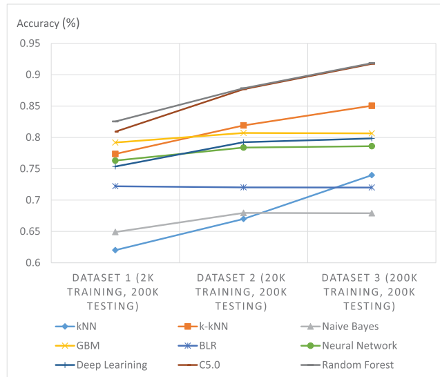
FIGURE 1. Detection Accuracy (%) of 9 Algorithms Using Dataset 1, 2 and 3 with the ratio of spams and non-spams being 1:1.
