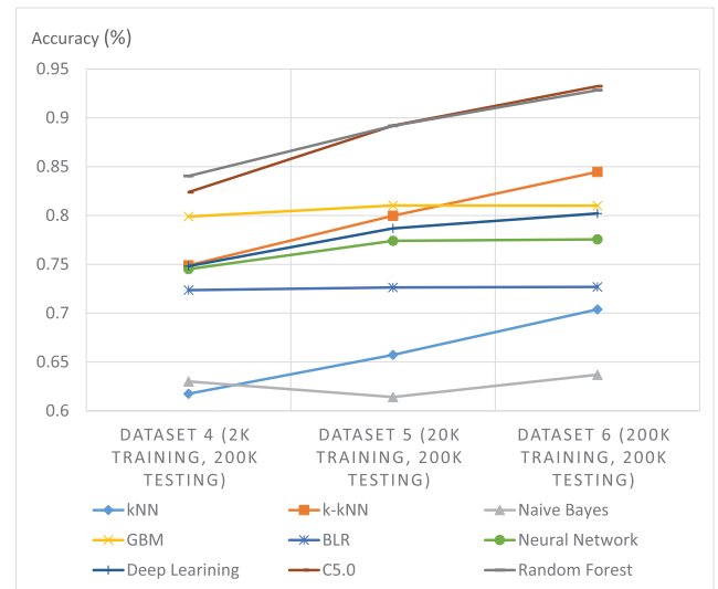
FIGURE 2. Detection Accuracy (%) of 9 Algorithms Using Dataset 4, 5 and 6 with the ratio of spams and non-spams being 1:19.
